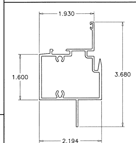
④ VENT TOP RAIL
