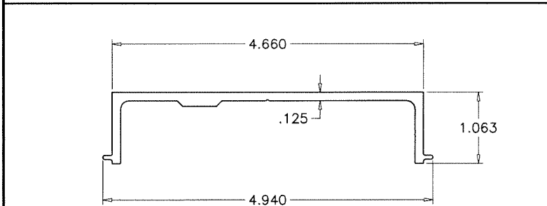
② INTERMEDIATE SILL
