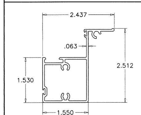
⑤ FIX. MEETING RAIL
