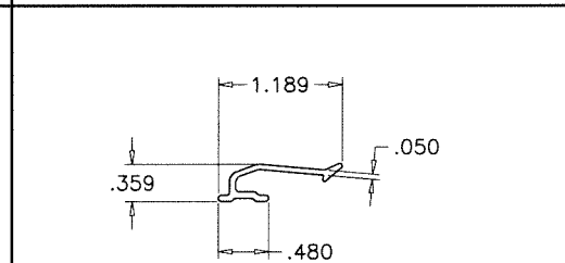
⑬ VENT STOP & VERTICAL COVER
