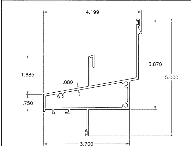
① FRAME HEAD/SILL
