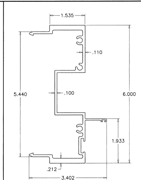
④ VENT TOP RAIL
