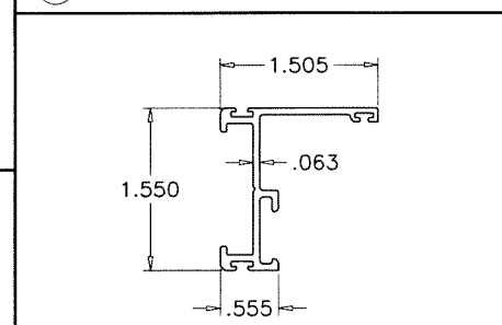
⑦ VENT SIDE RAIL
